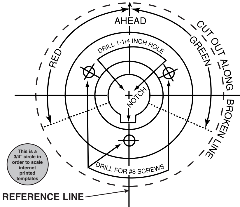
Fig. 1211 MOUNTING TEMPLATE
